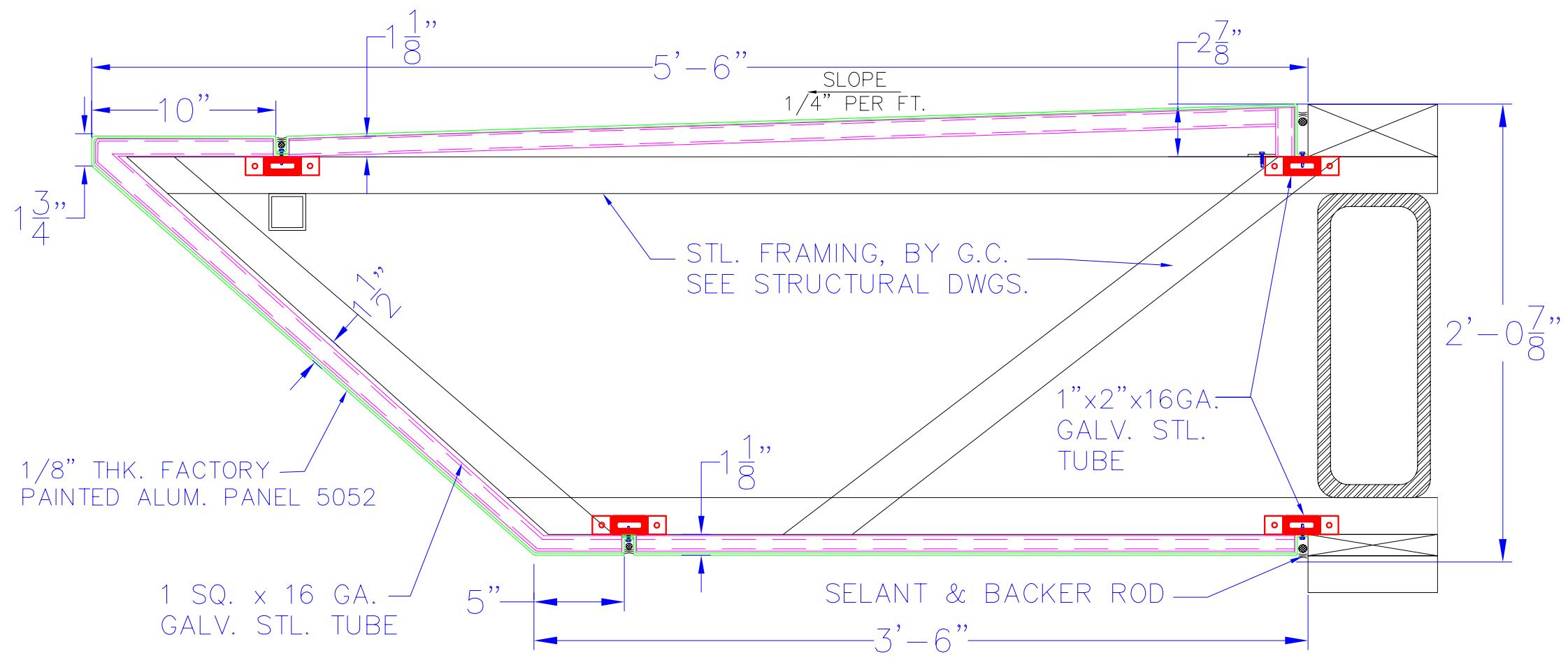
CANOPY SECTION B-B'
