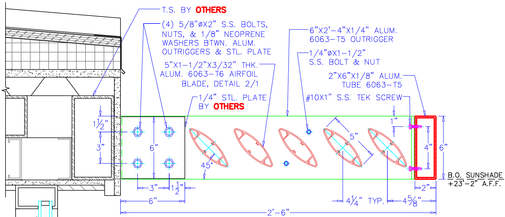
④ SUNSHADE SECTION
