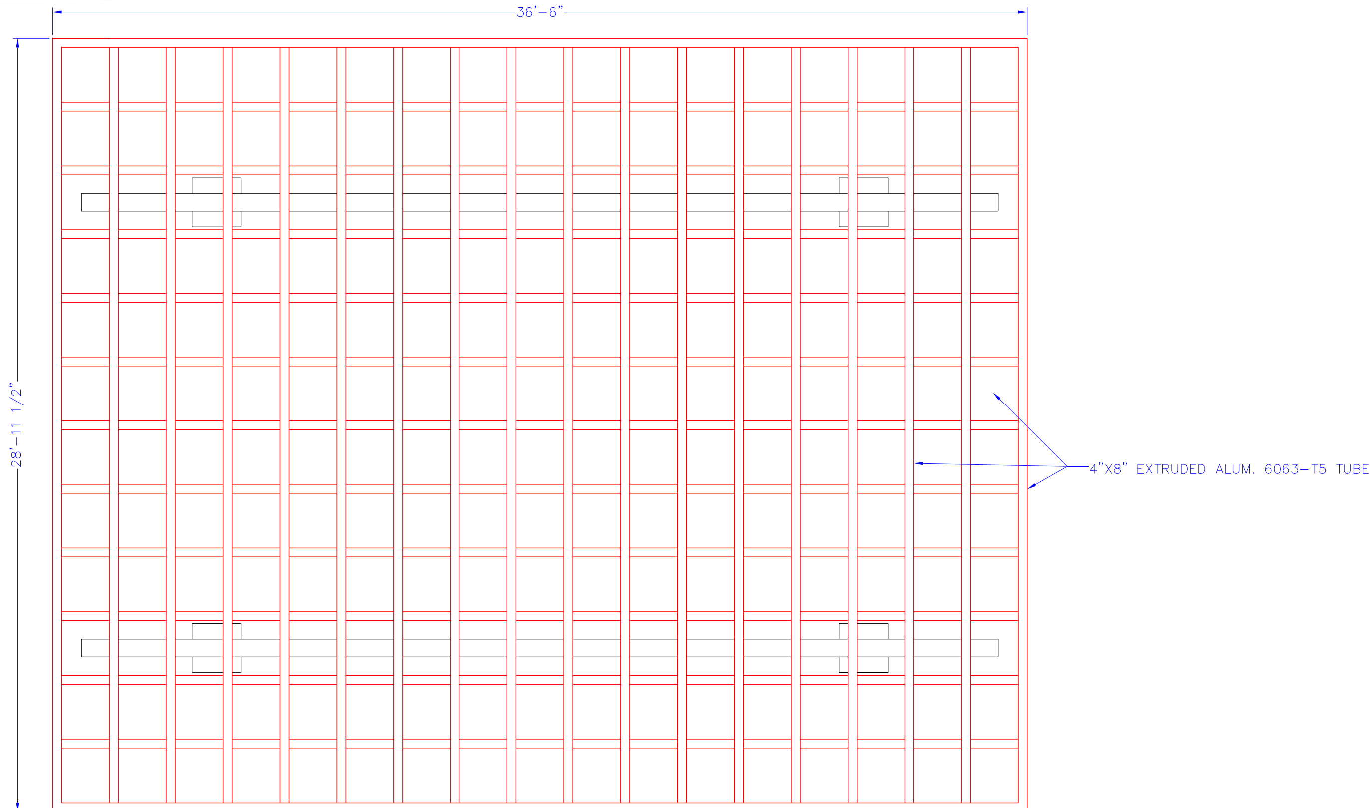
ALUM. TRELLIS - PLAN 1-UNIT: 28'-11 1/2" X 36'-6"
